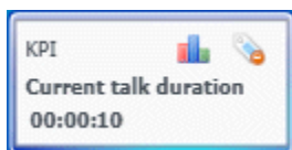
Tagged statistic
