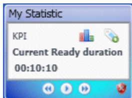
Statistics Gadget
